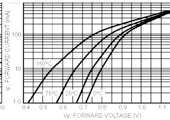
2. Typical Forward Voltage
