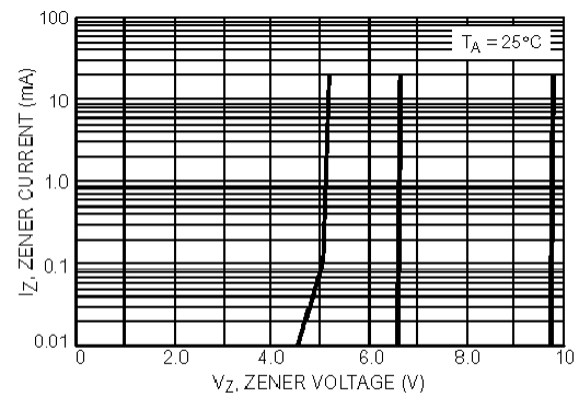
3. Zener Voltage versus Zener Current ( V_Z Up to 9 V)
